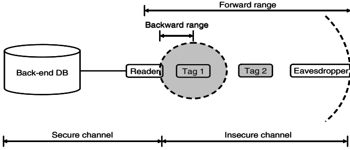
Fig. 1. RFID system
