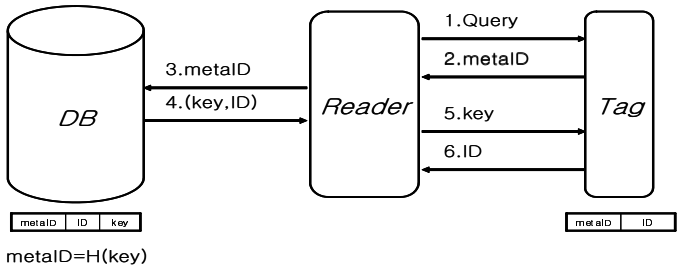
Fig. 2. The hash-lock protocol
