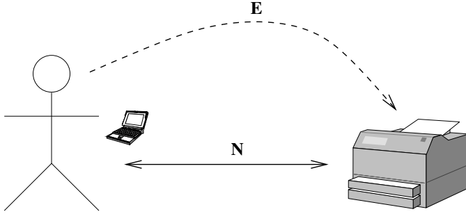
Fig. 3. Channel E now runs from user to printer, unobservable by the attacker. Channel N is bi-directional with the standard Dolev-Yao vulnerabilities
