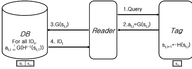
Fig. 4. The hash-chain protocol
