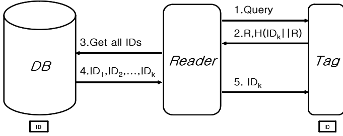
Fig. 3. The randomized hash-lock protocol
